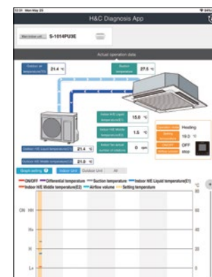
Refrigerant circuit view
